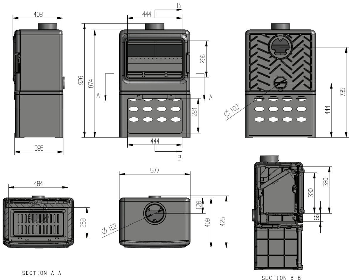
SECTION B-B
